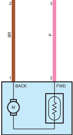
P4 Power Seat Motor (Driver's Seat Reclining Control)
