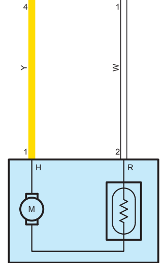
P5 Power Seat Motor (Driver's Seat Lumbar Support Control)
