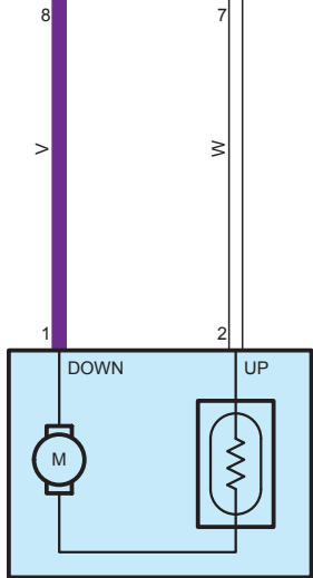
P2 Power Seat Motor (Driver's Seat Lifter Control)
