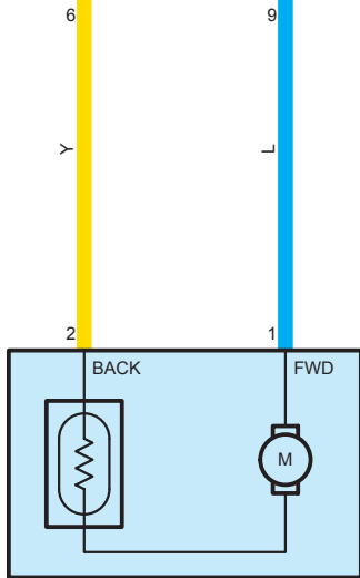
P1 Power Seat Motor (Driver's Seat Slide Control)
