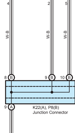
K22(A), P8(B) Junction Connector
