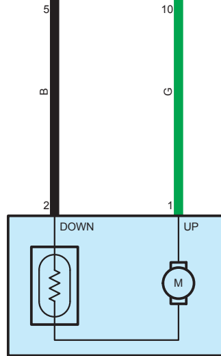
P3 Power Seat Motor (Driver's Seat Front Vertical Control)
